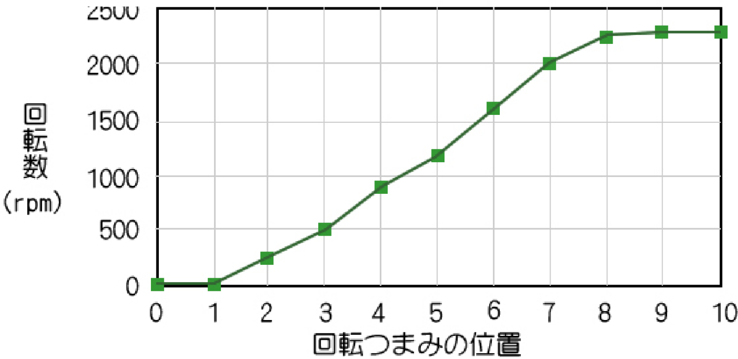
Rotation Speed vs. Control Knob Position
