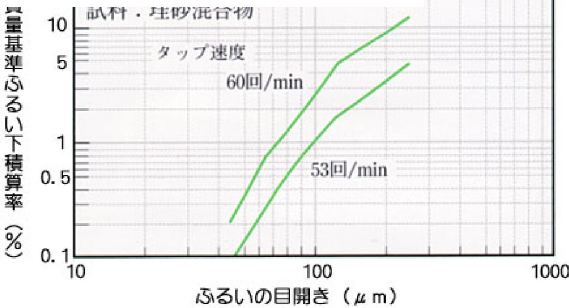
Example of Sieving Results
